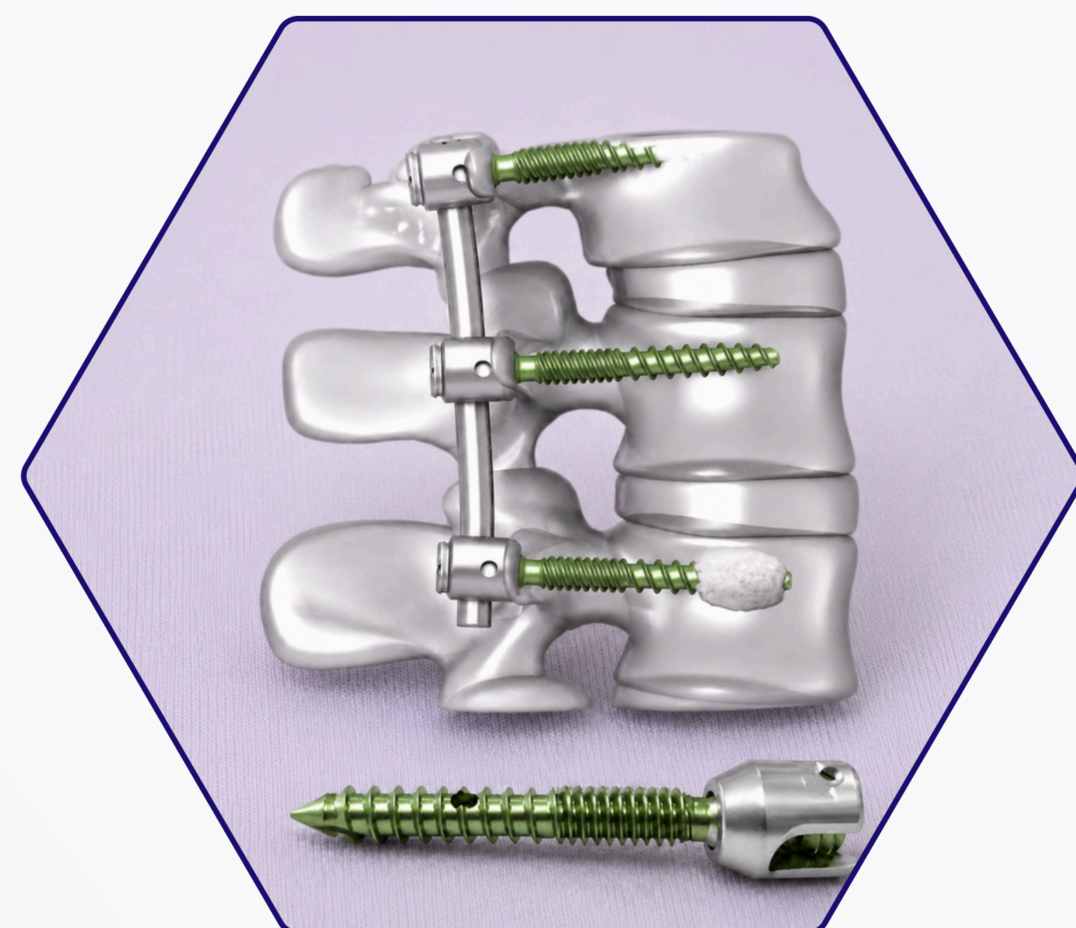
ARROW FENESTRATED SCREW
